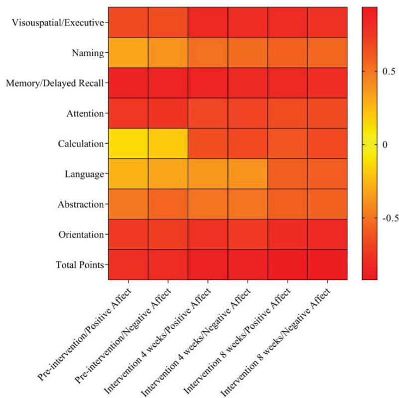
Fig. 1. Heat Map of the correlation between the degree of Cognitive Impairment and Emotional State in patients.
