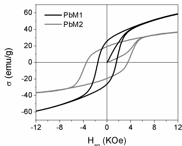
Figure 3. Hysteresis loops of the PBM1 and PBM2 samples.
