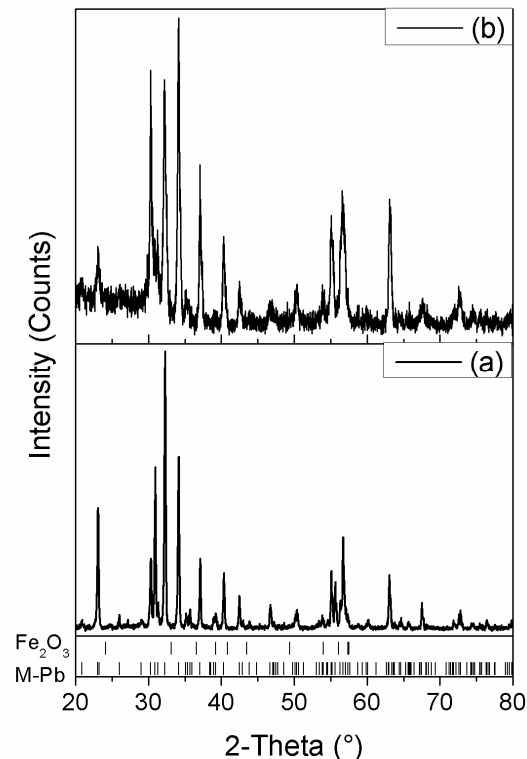
Figure 1. X-ray diffractogram of the sample prepared by a) the ceramic method (PBM1) and b) the coprecipitation method (PBM2).
